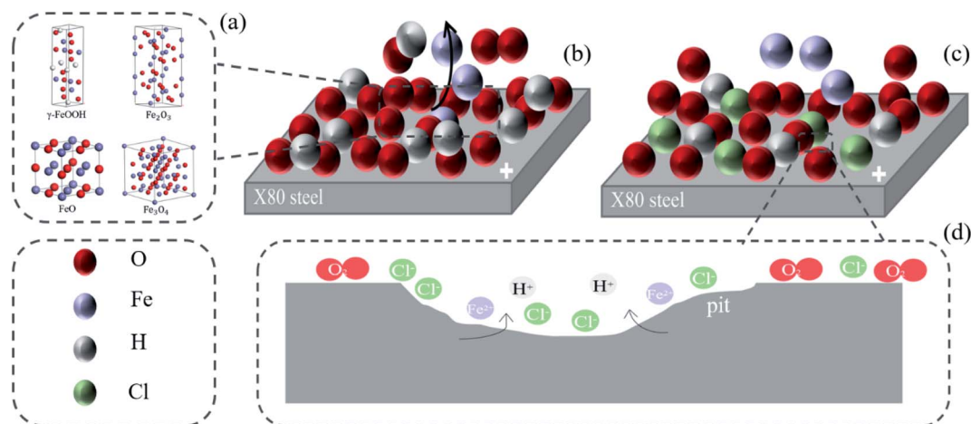
Fig. 14 Schematic representation of interface corrosion between X80 steel and chloride-containing pore solution: (a) the corrosion products, (b) the oxygen atom from lattice water molecules in the soil pore solution can get adsorbed on the metal surface atoms due to the high electronegativity of oxygen, (c) and (d) chloride ions feature the typical physical adsorption, under the electrostatic action, they can be characteristically adsorbed on the positively charged surface, and can get preferentially adsorbed on the defects of the metal crystal surface.
