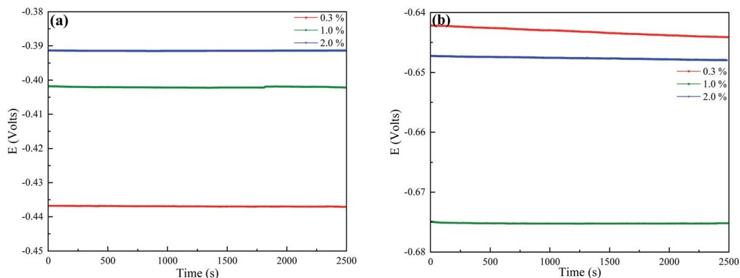
Fig. 10 Open circuit potential curves of X80 steel in various silty media: (a) NaCl and (b) \text{Na}_2\text{SO}_4 .
