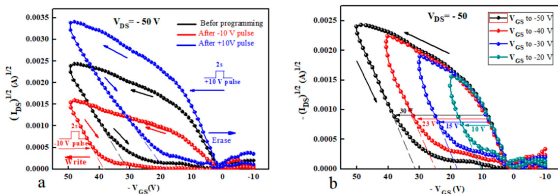
Figure 5. (a) Transfer characteristics of the fabricated OTFMT after the application of positive and negative pulses of 10 \text{ V} for 2 \text{ s} . (b) Double sweep of transfer characteristics of OTFMT with different maximum gate voltages.
