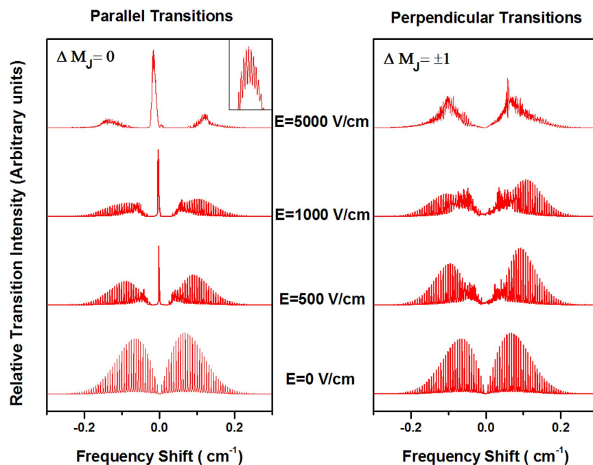
Figure 2. Calculated rotationally resolved spectrum of (\text{HCCCN})_3 molecule based on the molecular constants listed in Table 1. The lower abscissa scale is in \text{cm}^{-1} relative to the band origin of the vibrational mode of C-H stretch.
