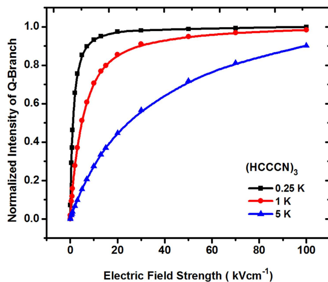
Figure 3. The dependences of the normalized Q-branch intensity on the E-field strength for different rotational temperature of (\text{HCCCN})_3 .
