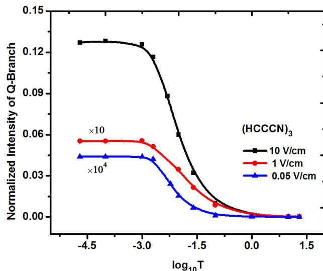
Figure 5. The dependences of the normalized Q-branch intensity on the rotational temperature of (HCCCN) 3 for different E-field strength. In which, the Y-coordinate values of the red and blue lines are multiplied by 10 times and 10000 times in order to compare with the black one; the line width of each possible transition is changed by 0.00001 cm -1 (≈B/300) to obtain higher resolution under 0.05 V cm -1 .
