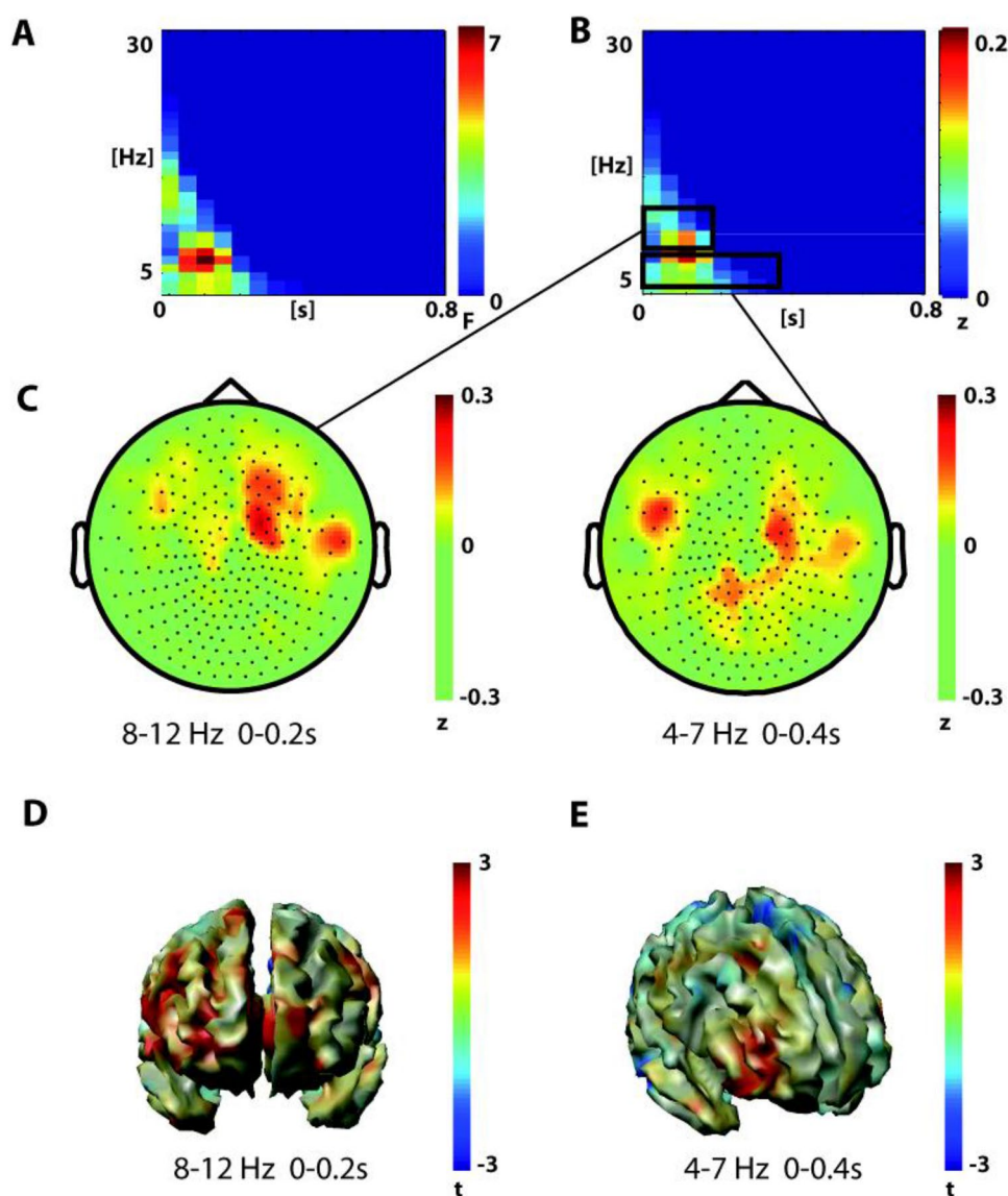
Fig. 4 Analysis of oscillatory power in the post-response interval (0 s to 0.8 s)—Main effect of Condition— anterior cluster a time–frequency representation of the anterior cluster in the main effect of condition (false alarms vs hits, 1-within 1-between permutation ANOVA, n = 26 , F-values masked by p < 0.05 , cluster correction, mean over significant channels shown). b Difference time–frequency representation for the significant cluster (false alarms minus hits). Black boxes mark two analysis windows. c, d Difference topographies (false alarms minus hits) in the significant cluster and both analysis windows marked in b . d, e Beamformer reconstructed source power of the two analysis windows of the anterior cluster of the main effect of condition in the post-response interval. The button is pressed at = 0 s
