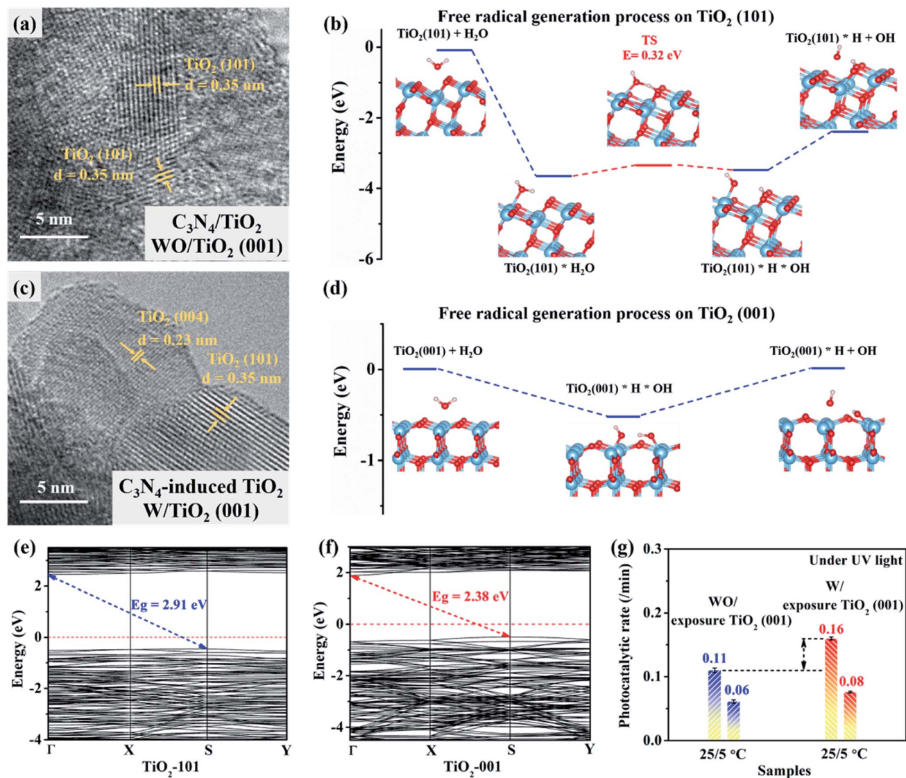
Fig. 2 Photocatalytic activity of samples with/without TiO_2(001) plane: HR-TEM images of each plane in (a) C_3N_4/TiO_2 and (c) C_3N_4 -induced TiO_2 . Simulated free radical generation process on (b) TiO_2(101) plane and (d) TiO_2(001) plane. Calculated band structures of (e) TiO_2(101) and (f) TiO_2(001) plane. (g) Comparative photocatalytic rates between C_3N_4/TiO_2 and C_3N_4 -induced TiO_2 under the UV light.
