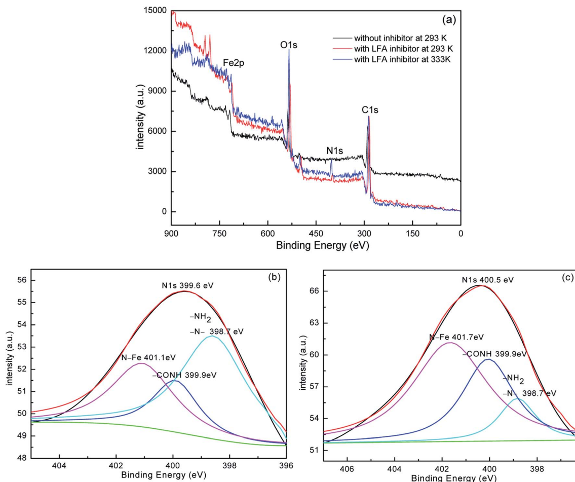
Fig. 12 XPS spectra of Q235 steel after 24 h immersion in \text{CO}_2 -saturated solution: (a) Wide-scan XPS spectra, (b) High-resolution spectra of N1s at 293 K and (c) 333 K.
