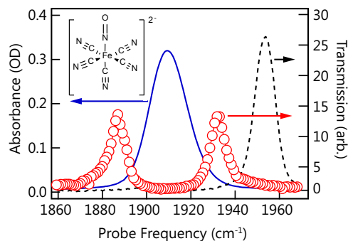
Fig. 1 Molecular structure and static spectra of SNP. The blue trace (left axis) is an absorption spectrum of SNP in MeOH in a CaF_2 transmission cell. The red trace (right axis) is the static transmission of the ultrafast infrared probe pulse through a 25\text{ }\mu\text{m} Fabry–Pérot cavity tuned to resonance with the NO stretching band. Open circles represent the pixel spacing of the detector. The black trace (right axis) is the transmission of the same cavity when the cavity mode is detuned from resonance with the NO stretching band. Inset is schematic of the SNP molecule.
