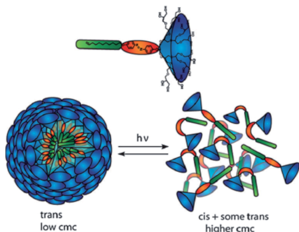
Fig. 22 Molecular structures of dendron amphiphiles (13a–13d) containing azo-benzene and proposed disruption of aggregates by light through trans – cis isomerization. Reprinted from ref. 69. Copyright 2011 Royal Society of Chemistry.
