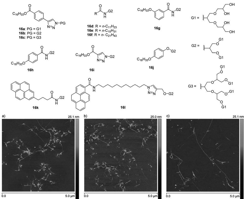
Fig. 25 Molecular structures of amphiphiles 16a–16l used for isolation and solubilization of CNTs and AFM images of SWNTs dispersed by amphiphiles 16b (a), 16f (b), and 16k (c). Adapted with permission from ref. 75. Copyright 2016 Wiley-VCH Verlag GmbH & Co. KGaA.
