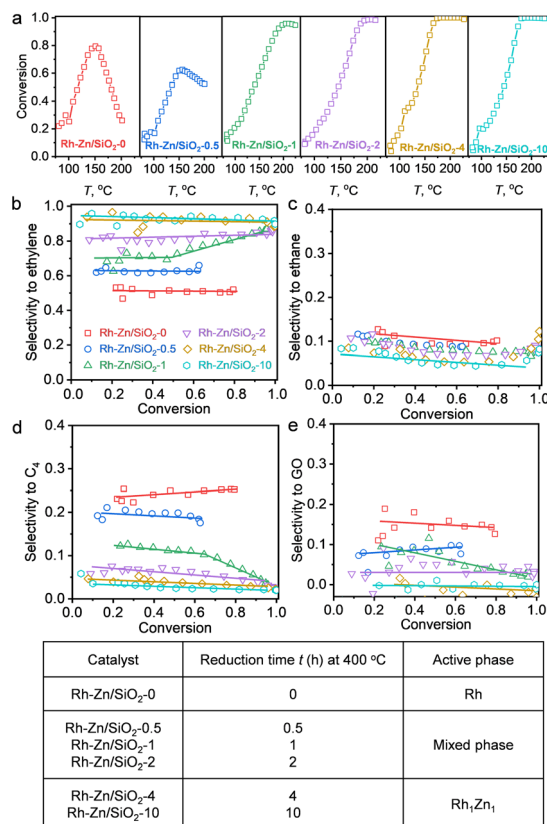
Fig. 3 Reduction time dependent catalytic performance of \text{Rh-Zn}/\text{SiO}_2 - t catalysts in acetylene hydrogenation. (a) Acetylene conversion over \text{Rh-Zn}/\text{SiO}_2 - t catalysts during temperature programmed reaction. Selectivity to (b) ethylene, (c) ethane, (d) \text{C}_4 and (e) GO versus acetylene conversion. (f) Relation between the denoted catalyst with the active phase. The product quantification was completed using GC (details of the calculation method are provided in the ESI†).
