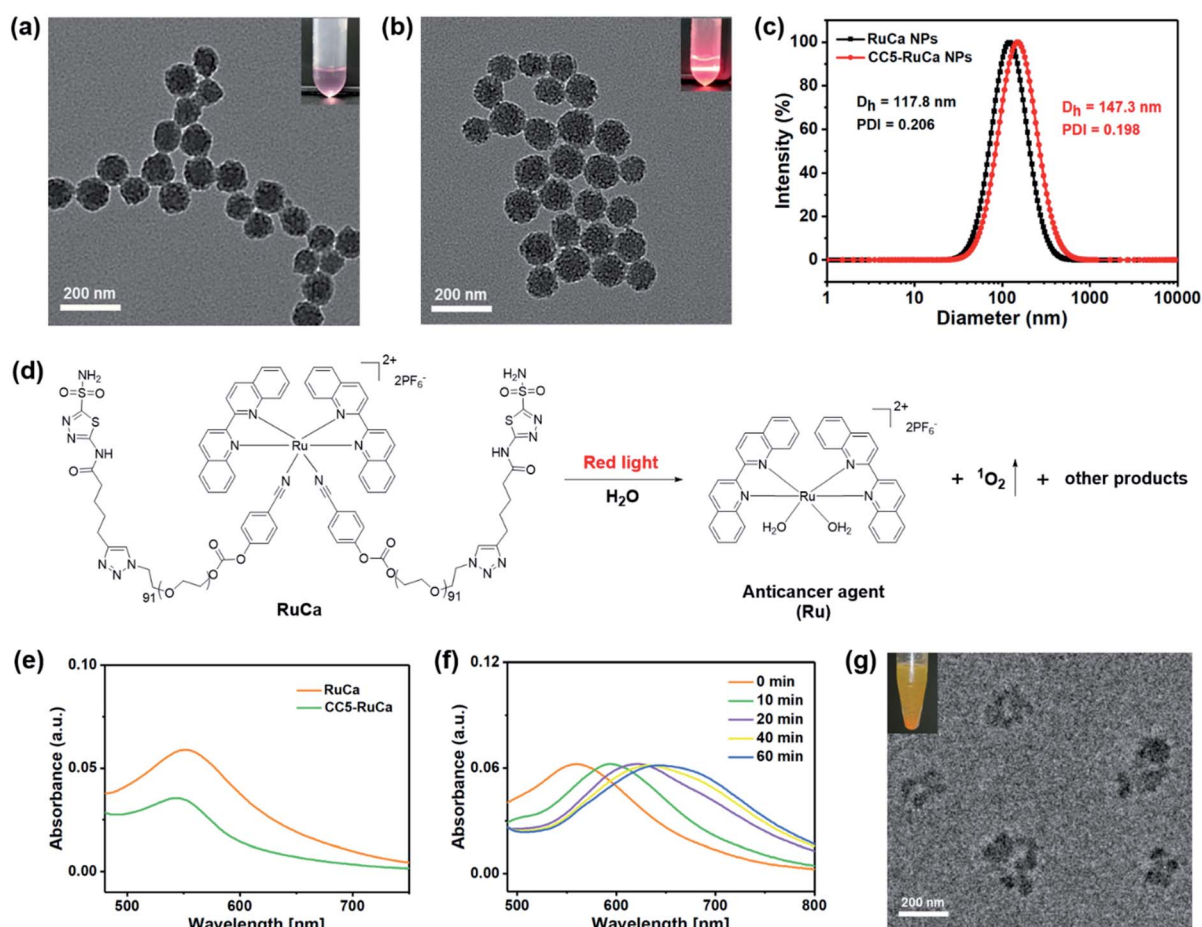
Fig. 4 TEM images of (a) RuCa and (b) CC5-RuCa NPs. Scale bar: 200 nm. (c) Hydrodynamic diameter of RuCa and CC5-RuCa NPs. (d) Red light ( 660 \text{ nm} , 30 \text{ mW cm}^{-2} ) induced degradation of RuCa. (e) UV-vis spectra of RuCa and CC5-RuCa NPs in water. (f) UV-vis absorption spectra of RuCa NPs under 660 \text{ nm} red light irradiation ( 30 \text{ mW cm}^{-2} ) for different time periods. (g) TEM image of RuCa NPs after 10 min laser irradiation. Scale bar: 200 nm.
