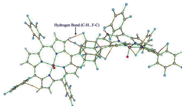
Fig. 3 Molecular graph of [(TPFPP)MnVO] 2 2+ which display C–H...F–C hydrogen bonds.
