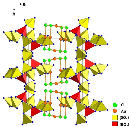
Figure 2. Crystal structure of [\text{Au}_3\text{Cl}_4][\text{B}(\text{S}_2\text{O}_7)_2] in projection on the ab -plane.
