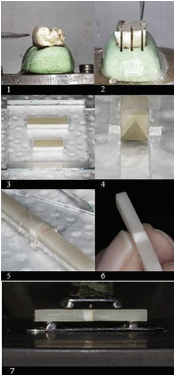
Fig. 1: Specimen preparation: 1.cutting the third of the crown 2.preparation of dentin blocks 3x4x3 3.precured composite blocks 4.attached dentin to composite 5.fixing the chevron with polyethel barrier 6.the uniform 3-part composite-dentin-composite. 7. 4-point test loading.
