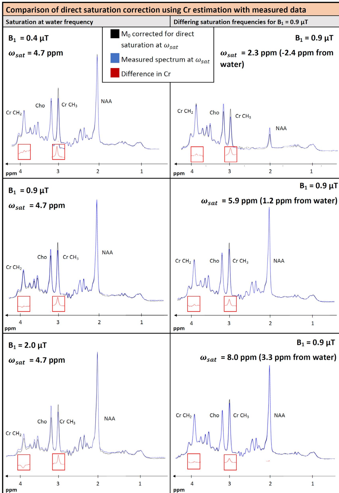
FIGURE 6 Comparison of the measured cohort-average spectra with M_0 spectra corrected for direct saturation at different B_1 values and saturation at the water frequency (left) and for a B_1 of 0.9 \mu\text{T} and different saturation frequencies (right). Direct saturation correction in this graph is based on values from Cr CH 3 . For saturation at the water frequency, the most prominent difference appears at the Cr CH 3 component. The Cr CH 2 peak does not show any difference. The prominent difference in Cr CH 3 decreases only a little when irradiating away from the water resonance. Only spectral features of Cr are drawn for the difference spectra because this plot only targets the \text{Cr}_{\text{tot}} peaks
