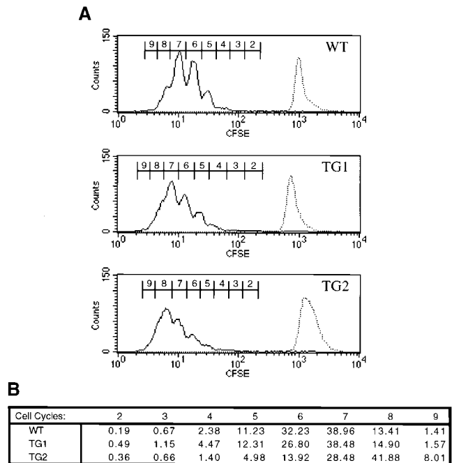
Figure 3. IFN- \gamma signaling does not affect the mitotic profile of Th1-polarized cultures. (A) CFSE-labeled, purified CD4 + splenocytes from WT, TG1, and TG2 mice (top, middle, and bottom, respectively) were cultivated on anti-CD3 plus anti-CD28-coated plates and Th1 polarized with anti-IL-4 mAbs and IL-12. 4 d after the initiation of the culture, cells were analyzed by flow cytometry for CFSE fluorescence gating on live CD4 + cells. The sequential dilution of intracellular fluorescein, depicted as peak progression from right to left, represents progressive cell division. The CFSE label intensity at the initiation of each culture is represented as a dashed histogram overlaid at the right of each panel. (B) A chart numerically representing the percentages of cells in each peak of the histograms in A. Results are representative of three independent experiments.
