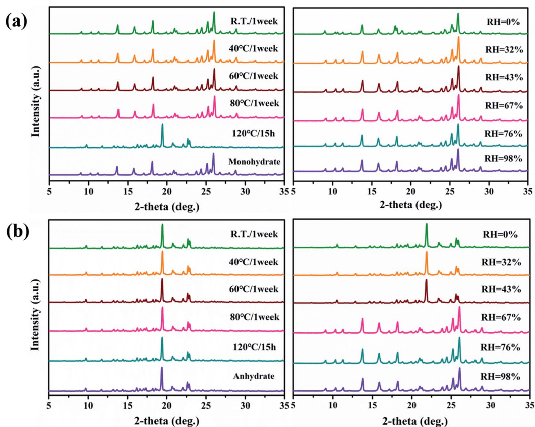
Fig. 10 The SST process of the monohydrate (a) and anhydrate (b) under different temperature and humidity conditions.
