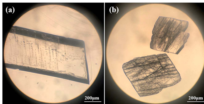
Fig. 3 Optical micrographs of crystals obtained in experiments: (a) monohydrate; (b) anhydrous form. The magnifications are 16× 10.
