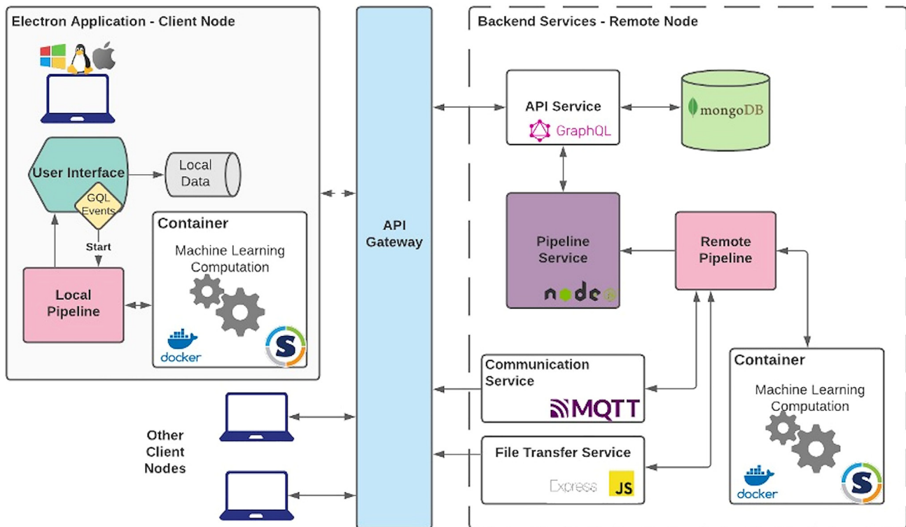
Figure 11. The COINSTAC architecture
