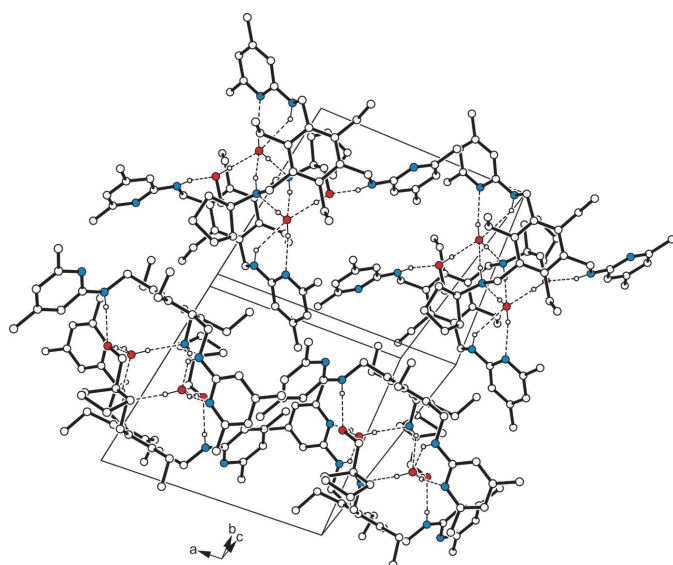
Figure 4 Packing diagram of 1a . Dashed lines represent hydrogen bonds. H atoms not involved in the hydrogen bonds are omitted.
