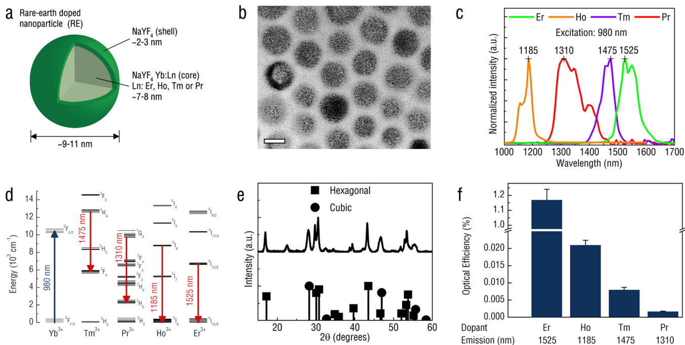
Figure 1. Properties of the rare-earth-doped nanoprobe
