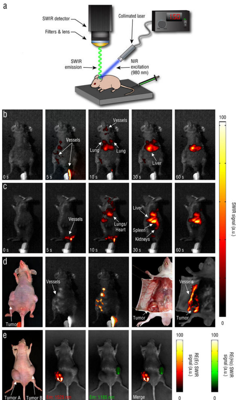
Figure 3. RE nanoprobes enable real-time and multispectral imaging in vivo Schematic of our portable SWIR-imaging prototype (a). The prototype consists of a room temperature cooled InGaAs camera operating at a typical exposure time of 50 ms, adjustable filter mounts, a collimated laser with an output power density of 0.14 \text{ W cm}^{-2} , and a neoprene rubber imaging surface. Real-time, video-rate biodistribution of intravenously injected REs captured in hairless mice using the imaging system prototype from both ventral (b) and left lateral (c) aspects. Nude mice bearing melanoma xenografts were intravenously injected with REs and imaged near surrounding tumor regions before dissection (d) from the
