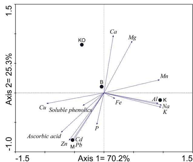
Fig. 4 Principal component analysis (PCA) biplot of sampling sites and heavy metal concentrations and ecophysiological parameters. M–Miasteczko Śląskie, B–Bukowno, K–Katowice-Kosztuchna, KO–Kokotek
