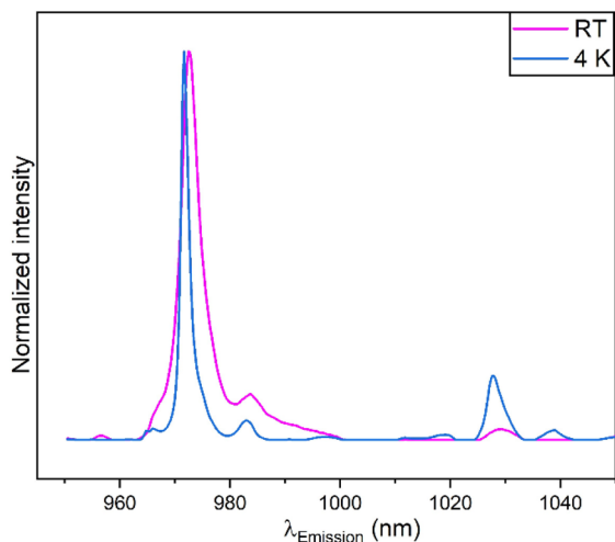
Fig. 9 Emission spectra of room temperature and 4 K measured 1273 K annealed samples (set 1, x \leq 0.05 ) obtained from PARAFAC analysis.
