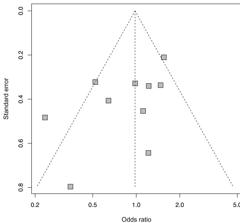
Figure 5 Funnel plot of the meta-analysis for the XPC rs2228001 polymorphism under the dominant model. Each gray square represents an included dataset. The vertical dashed line indicates the pooled odds ratio. The funnel defined by the two crossed dashed lines represents the pseudo 95% confidence interval.
