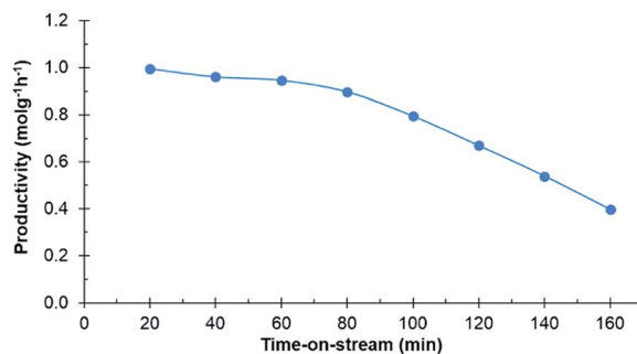
Fig. 4 Productivity of the catalyst in the continuous reactor over time-on-stream. Conditions: 0.1 \text{ mol l}^{-1} purified D -glucosone in \text{H}_2\text{O} ( 0.5 \text{ ml min}^{-1} ), 400 mg 0.7 wt% Ru/C catalyst, 20 bar \text{H}_2 ( 25 \text{ ml min}^{-1} ), 110^\circ\text{C} .
