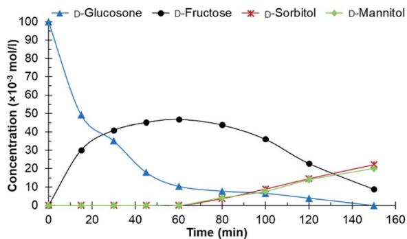
Fig. 1 Conversion of purified D -glucosone in the batch reactor. Conditions: 100 ml 0.1 \text{ mol l}^{-1} purified D -glucosone in \text{H}_2\text{O} , 100 mg 4.6 wt% Ru/C catalyst, 20 bar \text{H}_2 , 110^\circ\text{C} .
