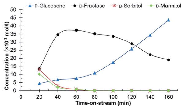
Fig. 3 The conversion of D -glucosone in the continuous reactor. Conditions: 0.1 \text{ mol l}^{-1} purified D -glucosone in \text{H}_2\text{O} ( 0.5 \text{ ml min}^{-1} ), 400 mg 0.7 wt% Ru/C catalyst, 20 bar \text{H}_2 ( 25 \text{ ml min}^{-1} ), 110^\circ\text{C} .
