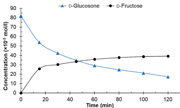
Fig. 2 Conversion of crude D -glucosone in the batch reactor. Conditions: 100 ml 0.08 \text{ mol l}^{-1} crude D -glucosone in \text{H}_2\text{O} , 100 mg 4.6 wt% Ru/C catalyst, 20 bar \text{H}_2 , 110^\circ\text{C} .
