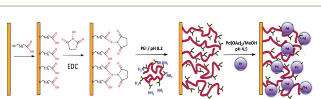
Scheme 1 Palladium immobilization on polyethylenimine coated Au/quartz surfaces.
