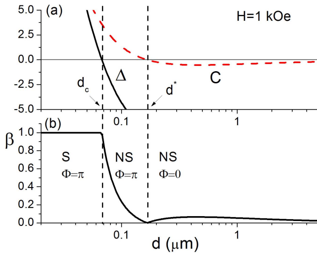
Figure 6 | (a) Criterion for phase transition \Delta and interaction coefficient C as a function of thickness d for fixed magnetic field H = 1 kOe. (b) The contrast \beta = \frac{|\Psi_{\max}^2 - |\Psi_{\min}^2|}{|\Psi_{\max}^2 + |\Psi_{\min}^2|} as a function of thickness d for H = 1 kOe. S and NS denote symmetric and non-symmetric state, respectively.
