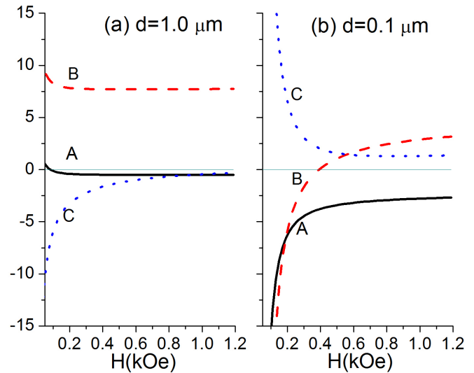
Figure 2 | The interaction coefficients A , B and C (in units of \text{mK/N} , with N the total number of spins in the film) as a function of magnetic field H for film thickness (a) d = 1.0 \mu\text{m} and (b) d = 0.1 \mu\text{m} .
