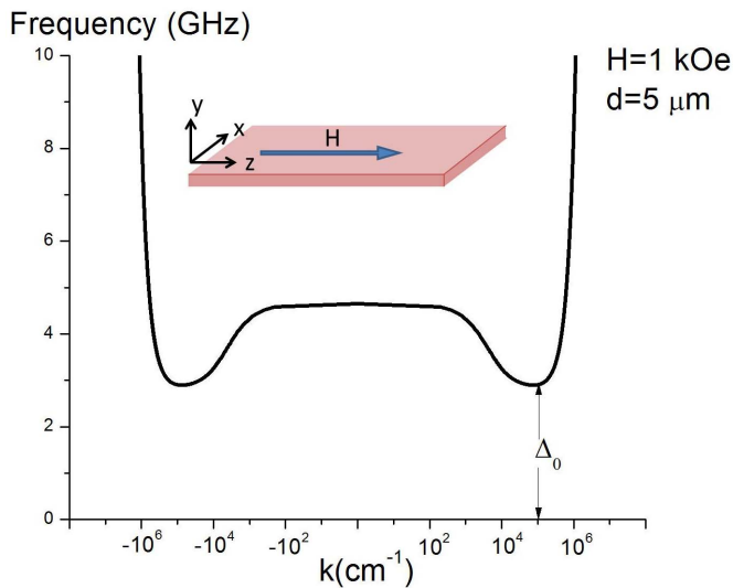
Figure 1 | The magnon spectrum in the k_z direction for d = 5 \mu\text{m} and H = 1 \text{ kOe} . The inset is a schematic diagram of YIG film.
