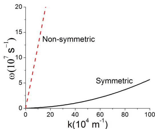
Figure 5 | Dispersion of zero sound as a function of wave vector in the direction of external magnetic field for symmetric and non-symmetric states, respectively. For the non-symmetric state, we choose H = 1 \text{ kOe} and d = 5 \text{ μm} .
