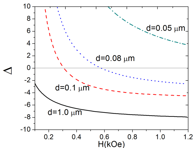
Figure 3 | The criterion of transition from non-symmetric to symmetric phase, \Delta (in units of mK/N), as a function of magnetic field H for different values of thickness d .
