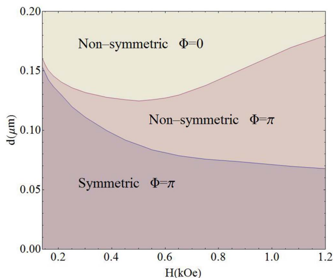
Figure 4 | The phase diagram for different values of thickness d and magnetic field H .
