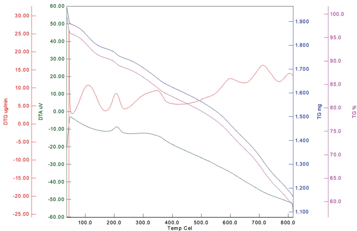
Fig. 5 TGA pattern of \text{Fe}_3\text{O}_4@YSPMO@Ru .
