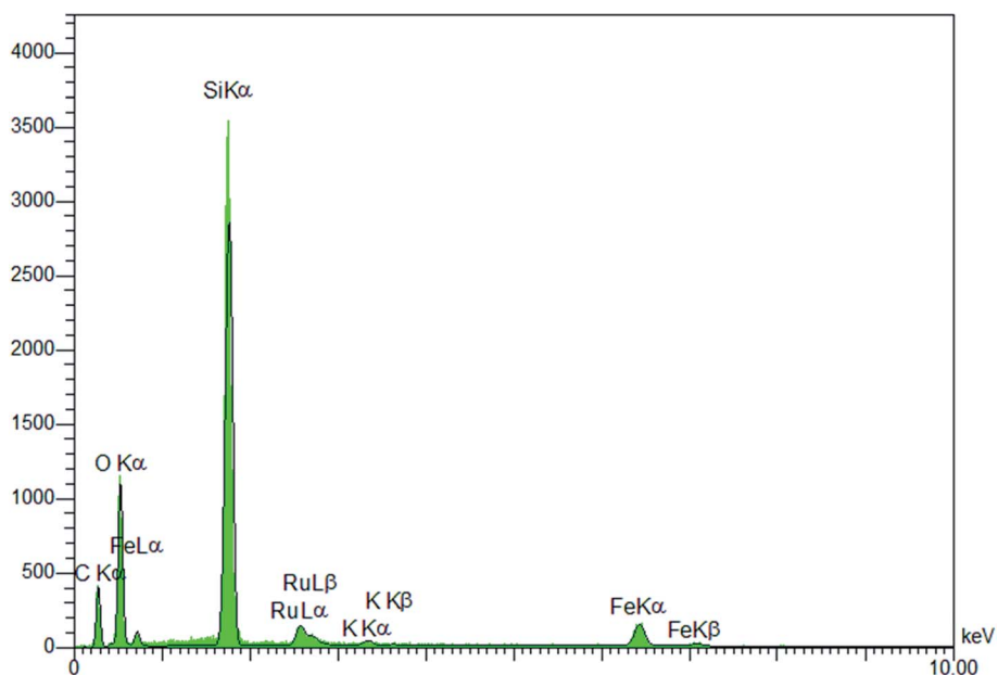
Fig. 6 EDS spectrum of \text{Fe}_3\text{O}_4@YSPMO@Ru .
