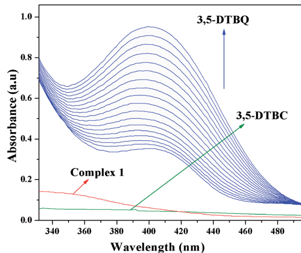
Fig. 9 Time resolved UV-Vis spectral profiles indicating the increment of 3,5-DTBQ peak at \sim 400 nm upon addition of 10^{-2} M 3,5-DTBC to the 10^{-4} M of complex 1 in acetonitrile–methanol (2 : 1) mixture at room temperature.
