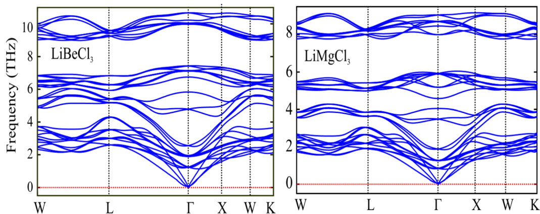
Fig. 3 The computed phonon band spectra of \text{LiBeCl}_3 and \text{LiMgCl}_3 ternary chloroperovskites compounds.
