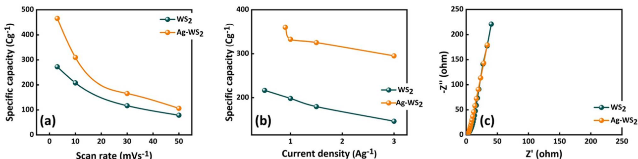
Fig. 5 (a) Specific capacity from CV, (b) specific capacity from GCD and (c) EIS of WS 2 and Ag-WS 2 .
