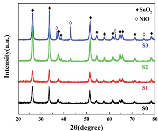
Fig. 3 PXRD patterns of pure and Ni-doped SnO 2 .
