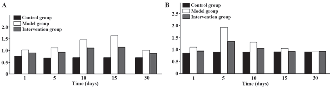
Figure 3. Expression levels of coxsackie-adenovirus receptor (CAR) and p38 mitogen activated protein kinase (MAPK) at different time-points tested by western blot analysis (A) CAR and (B) p38 MAPK.
