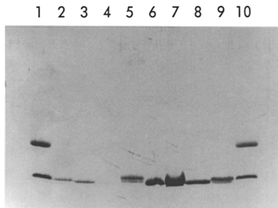
Figure 3. Urea-SDS-PAGE of purified neutrophil-activating peptides. Molecular mass markers aprotinin (6.5 kD) and lysozyme (14.4 kD) (lanes 1 and 10), active peptide from pool P1 (49.3-min peak) (lane 2), GRO \alpha (lane 3), GRO \gamma (lane 4), IL-8 (77 aa) (lane 5), three preparations of ENA-78 (lanes 6-8), and recombinant IL-8 (lane 9).
