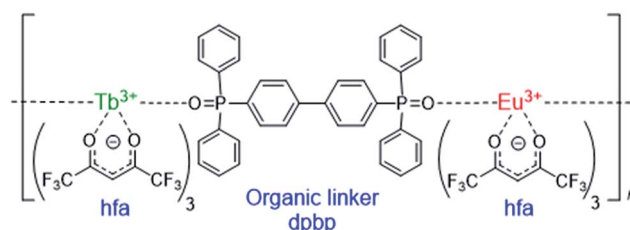
Fig. 1 Chameleon thermometer [Ln(hfa) 3 (dpdp)] n (Ln = Eu and Tb).
