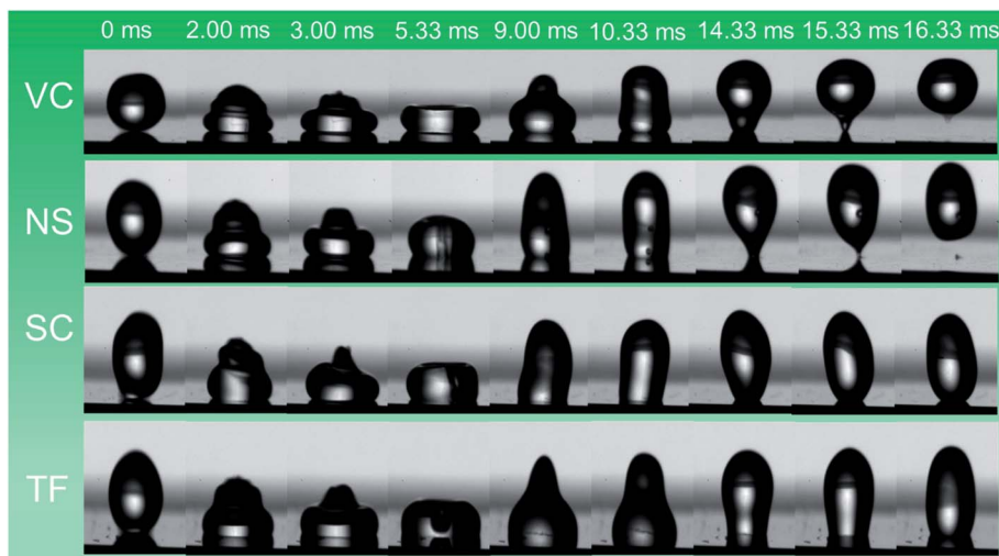
Fig. 3 Time evolution of 10 \mu\text{L} water droplets dropped from a height of 10 mm on different nanostructures (ESI). † Water droplet bouncing was observed on vertical columns and nanospring samples. The water droplet rebounded on VC and NS and left the surface in approximately 16 ms.
