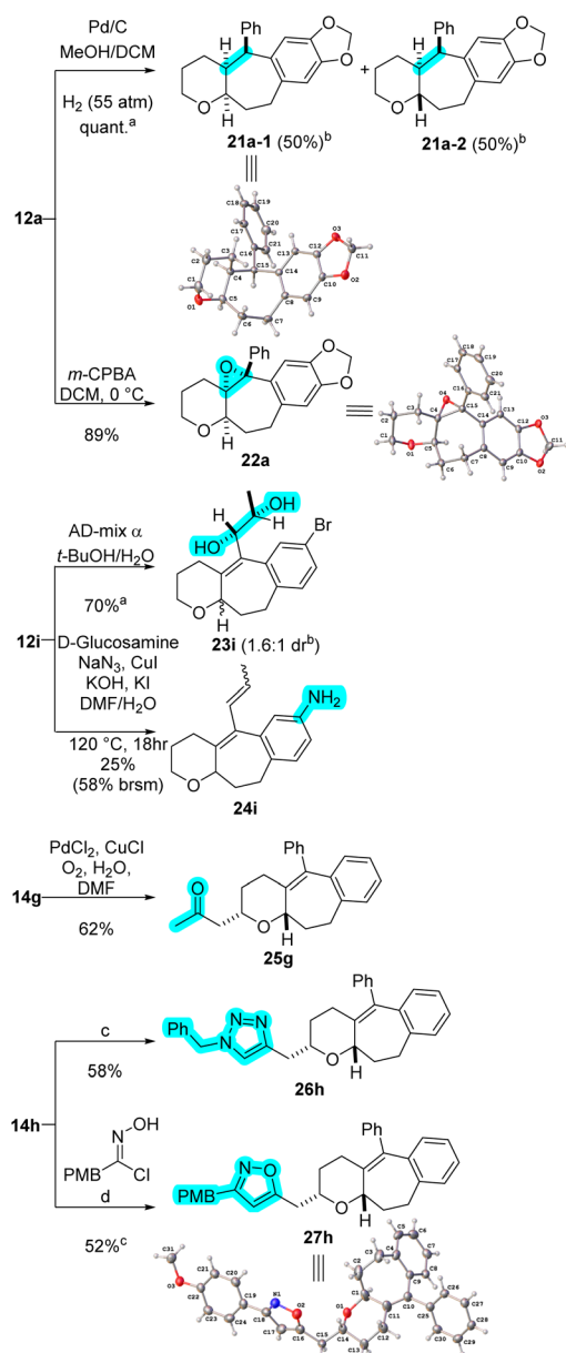
Scheme 8 Diversification of cycloadducts. (a) Combined yield of two diastereomers (b) dr determined based on isolated yields of separable diastereoisomers (c) \text{BnN}_3 , Cu powder, \text{CuSO}_4 \cdot 5\text{H}_2\text{O} , sodium ascorbate, \text{H}_2\text{O}/t\text{-BuOH} , rt. (d) Cu powder, \text{CuSO}_4 \cdot 5\text{H}_2\text{O} , \text{NaHCO}_3 , \text{H}_2\text{O}/t\text{-BuOH} , rt.
