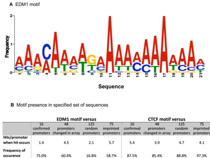
Figure 6. Identification of a DNA sequence motif EDM1 (Environmental Induced Differential Methylation Consensus Sequence 1). (a) Logo representation of the motif EDM1. This motif was obtained with the GLAM2 tool of MEME suite from the set of 16 regions that had been confirmed with mass spectrometry to present transgenerational changes in methylation. Glam2 score value for this motif is 194.184 (b) Results obtained when scanning EDM1 with GLAM2SCAN for prevalence of matches against four sets of sequences: (i) the 16 promoters containing the regions positively confirmed to be changed, (ii) the 48 promoters containing the regions confirmed to show change in the array, (iii) a set of 125 random promoters, and (iv) a set of 75 imprinted promoter regions from mouse and rat databases. Results shown are from matches in GLAM2SCAN scoring equal or higher than the cut-off value of 20. doi:10.1371/journal.pone.0013100.g006
