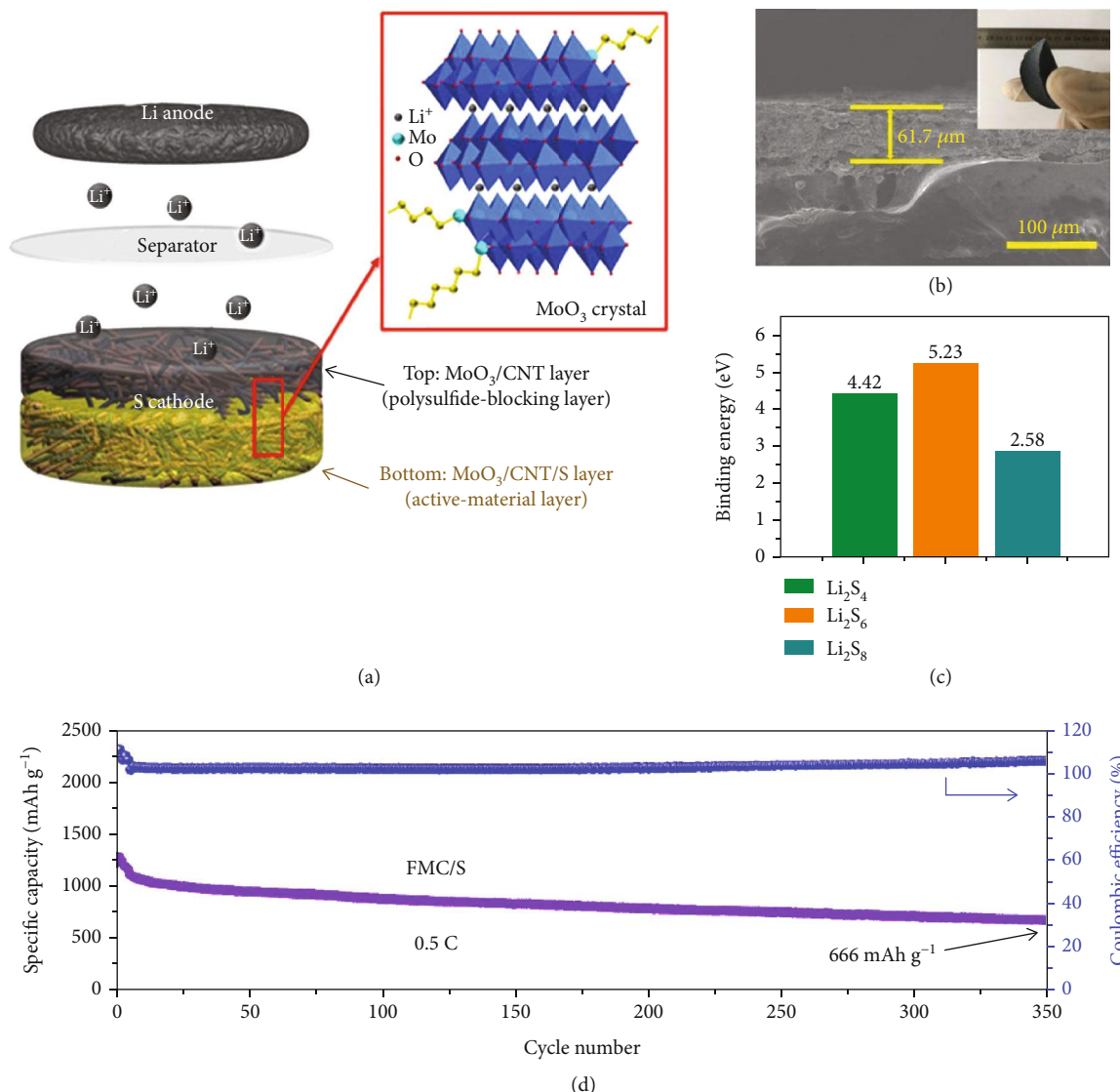
FIGURE 4: (a) Li-S battery adopting freestanding MoO 3 /CNT/S (FMC/S) as the cathode. (b) Cross-sectional observation of the FMC/S membrane. Inset: bending test of the FMC/S membrane. (c) The calculated binding energies between MoO 3 and LiPSs (including Li 2 S 4 , Li 2 S 6 , and Li 2 S 8 ). (d) Cycling stability of the FMC/S at 0.5 C. (a–d) Reproduced with permission from the American Chemical Society [52].
