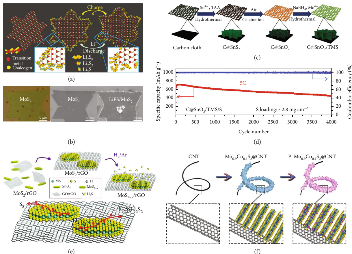
FIGURE 8: (a) Schematic illustration for the confined deposition and conversion of LiPSs at the preferential catalytic sites of transition metal dichalcogenide (TMD) nanosheets. (b) Optical and SEM images of \text{MoS}_2 flakes and LiPS-deposited \text{MoS}_2 flakes at the discharged state. (a, b) Reproduced with permission from the American Chemical Society [69]. (c) The synthesis of the hierarchical \text{C@SnO}_2/\text{TMS} nanoarray on carbon cloth. (d) Long-term cycling stability test of the \text{C@SnO}_2/\text{TMS}/\text{S} cathode at 5C. (c, d) Reproduced with permission from the American Chemical Society [70]. (e) The synthesis of \text{MoS}_{2-x}/\text{rGO} and the conversion of \text{Li}_2\text{S}_x . Reproduced with permission from the Royal Society of Chemistry [71]. (f) The synthesis of cobalt (Co) and phosphorus (P) codoped \text{MoS}_2 ( \text{P-Mo}_{0.9}\text{Co}_{0.1}\text{S}_2 ) on CNT. Reproduced with permission from Wiley-VCH [72].
