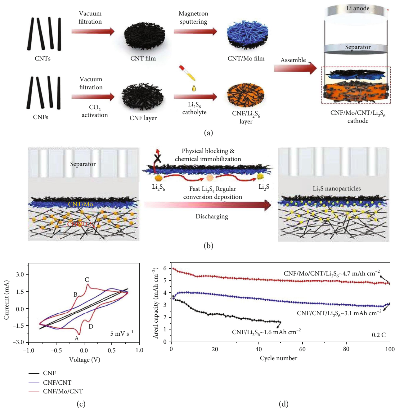
FIGURE 19: (a) The assembly of the Li-S battery based on the CNF/Mo/CNT/ \text{Li}_2\text{S}_6 cathode. (b) The electrochemical behavior of the CNF/Mo/CNT/ \text{Li}_2\text{S}_6 cathode with the \text{Li}_2\text{S}_6 catholyte. (c) CV curves of the symmetric cells employing CNF/Mo/CNT, CNF/CNT, and CNF electrodes at 5 \text{ mV s}^{-1} . (d) Cycling performances of Li-S batteries based on CNF/Mo/CNT/ \text{Li}_2\text{S}_6 , CNF/CNT/ \text{Li}_2\text{S}_6 , and CNF/ \text{Li}_2\text{S}_6 electrodes under a high sulfur mass loading ( 7.6 \text{ mg cm}^{-2} ). (a–d) Reproduced with permission from the American Chemical Society [118].
