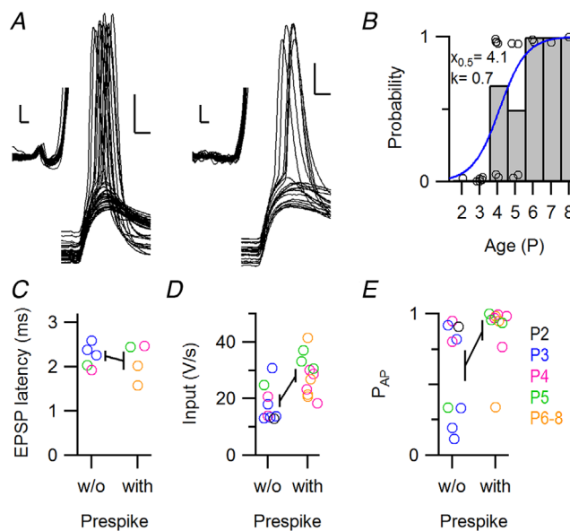
Figure 3. Comparison of strong inputs with and without prespikes
