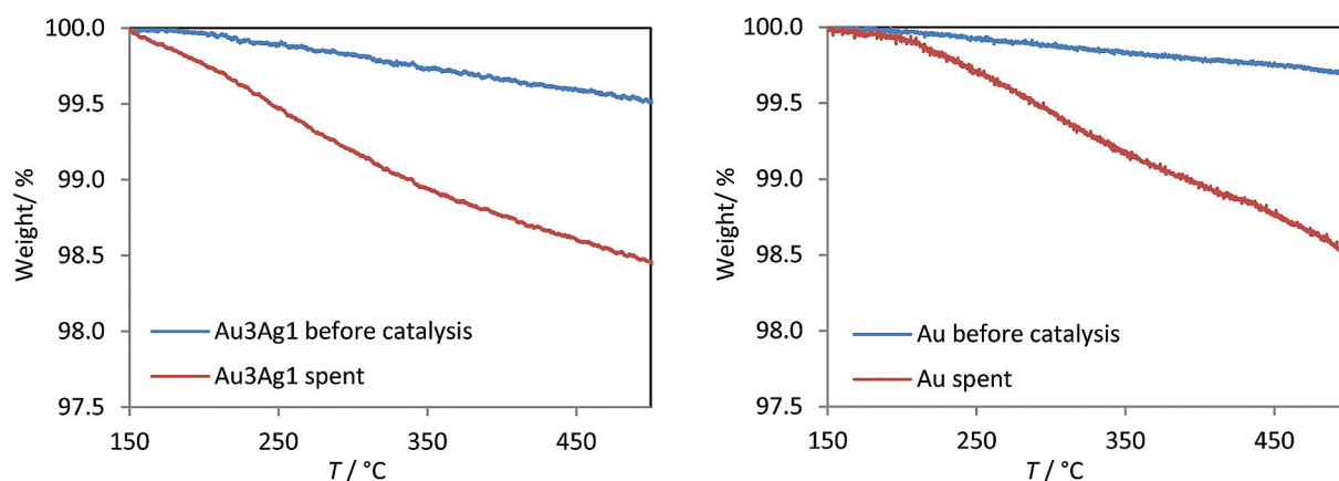
Figure 6. Mass loss of the Au3Ag1 (left) and Au (right) samples during heating with 5 °Cmin -1 under a 10 mLmin -1 flow of oxygen.
