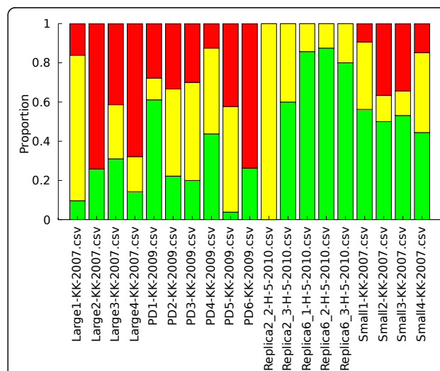
Figure 5 Distribution of experimental adaptive events. The relative proportions of adaptive events in each subpopulation, calculated using the PSM, in the three chemostat systems considered here. The neutrality of the fluorescent proteins implies that there should not be a consistent bias of adaptive events towards any particular color, and this assumption holds here for all chemostats. Statistically significant differences in adaptive event abundance between the labeled populations would imply the presence of jackpot mutants.
