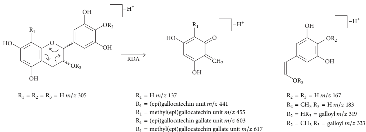
FIGURE 5: Characteristic fragments obtained from Retro-Diels-Alder (RDA) fission of a prodelphinidin.
