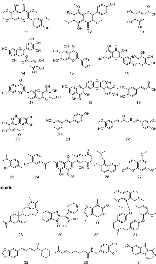
Fig. 3. Chemical structures of some potent efflux pump inhibitors derived from edible plants.
