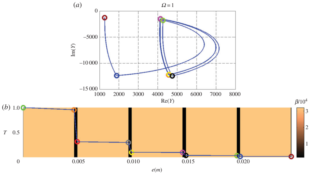
Figure 4. Nine-layer stack at pulsation \omega = 1 Hz, with the admittance diagram in the complex plane (a) and the distribution of temperature modulus (b). See text for all scales.
