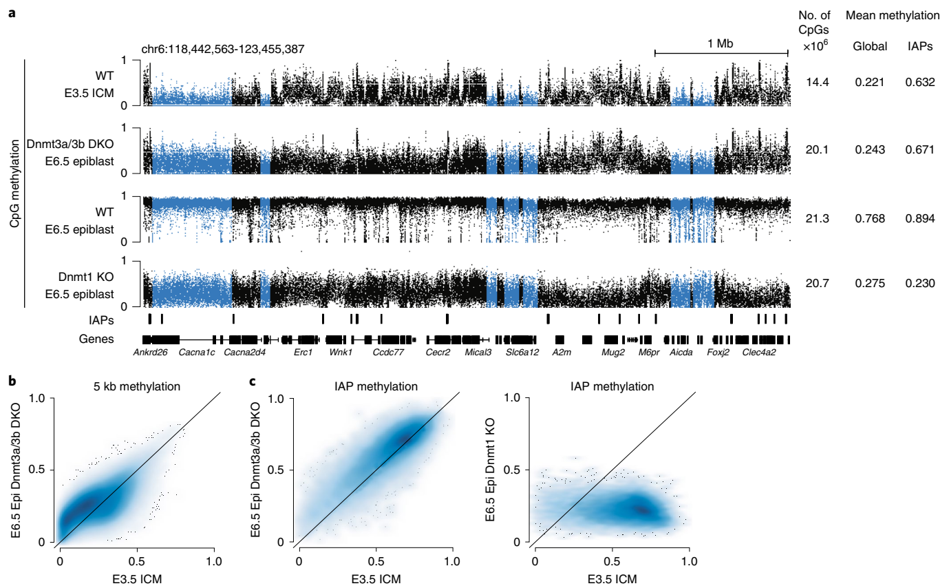
Fig. 1 | Dnmt1 displays de novo methylation activity in vivo. a , Representative genome browser tracks of WGBS data for WT E3.5 ICM ( n=2 samples from 5–10 pooled embryos each), Dnmt3a/3b DKO E6.5 epiblast ( n=1 from ~10 pooled embryos each), WT E6.5 epiblast ( n=2 from ~10 pooled embryos each) and Dnmt1 KO E6.5 epiblast ( n=1 from ~10 pooled embryos each). Regions with a notable gain of methylation in the absence of the de novo Dnmt3s are highlighted across all tracks in blue. The coverage and average methylation values are shown on the right. b , Correlation plot of E3.5 ICM compared to E6.5 epiblast (Epi) of the Dnmt3a/3b DKO in 5-kb windows, excluding all IAP retrotransposon overlapping CpGs. n=461,268 5-kb windows. c , Correlation plot of the average IAP retrotransposon methylation per element in the E3.5 ICM compared to E6.5 epiblast of the Dnmt3a/3b DKO (left) and Dnmt1 KO (right); 48% of IAPs are more methylated ( >0.05 methylation difference) than in the ICM of Dnmt3a/3b DKO epiblast and almost all (96%) are less methylated in the Dnmt1 KO than in the ICM. n=14,787 IAP elements. Source data are provided at https://doi.org/10.6084/m9.figshare.14555250 .
