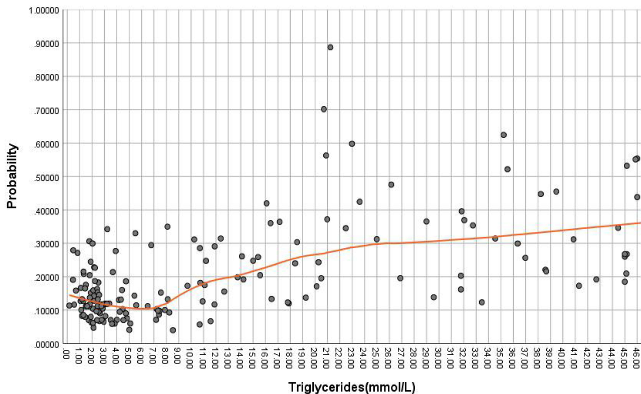
Figure 4 Observed and expected incidence of SAP in patients with different triglycerides concentrations. Notes: The black circles give the observed incidence of SAP for each patient. The solid curve gives expected incidence of SAP based on restricted cubic spline analysis. Abbreviation: SAP, severe acute pancreatitis.
