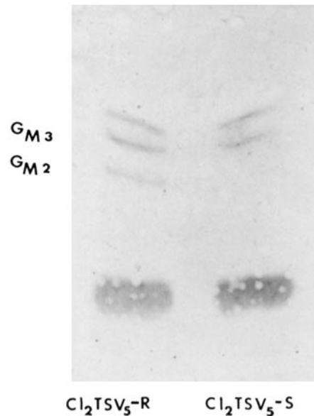
FIGURE 2 Photograph of a thin-layer chromatogram of gangliosides isolated from reaction mixtures containing Cl 2 TSV 5 -S (right) and Cl 2 TSV 5 -R (left) cells incubated for 3 h in the presence of UDP- N -acetylgalactosamine and BHK hematoside. The composition of the reaction mixture, the isolation of gangliosides, and conditions for the development of the chromatogram are given in Materials and Methods and in Fig. 1. The amount of protein in the extracts was 200 μg in each case.
