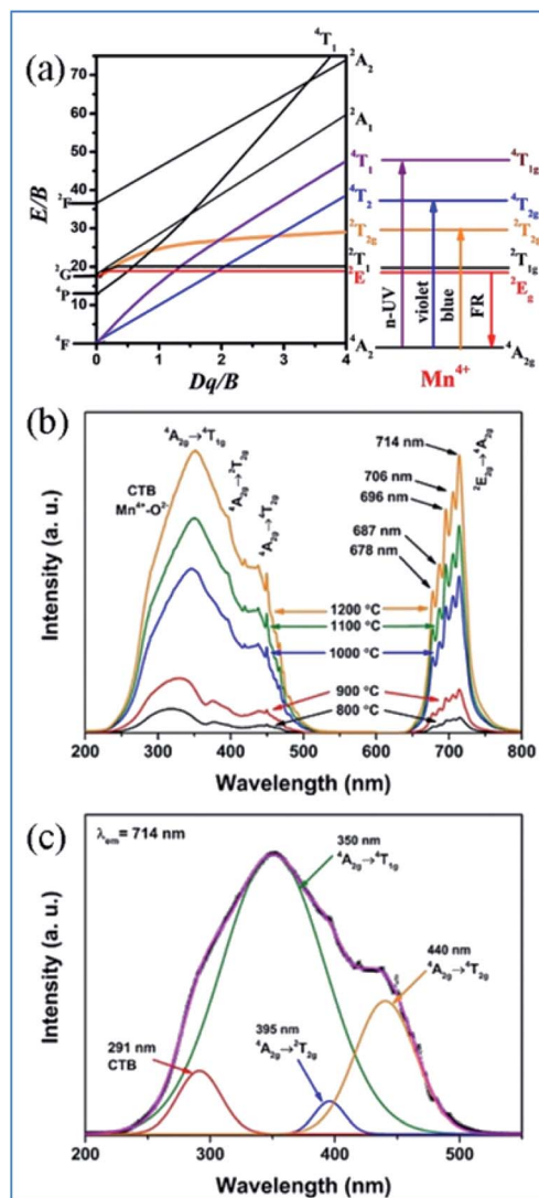
Fig. 3 (a) Tanabe–Sugano diagram for Mn 4+ dependent on the crystal field in complex oxides, (b) typical PLE and PL spectra, and (c) Gaussian curves of PLE spectra of Mn 4+ in Ca 14 Zn 6 Ga 10 O 35 phosphors. Reprinted with permission from ref. 39, Copyright 2017, The Royal Society of Chemistry.
