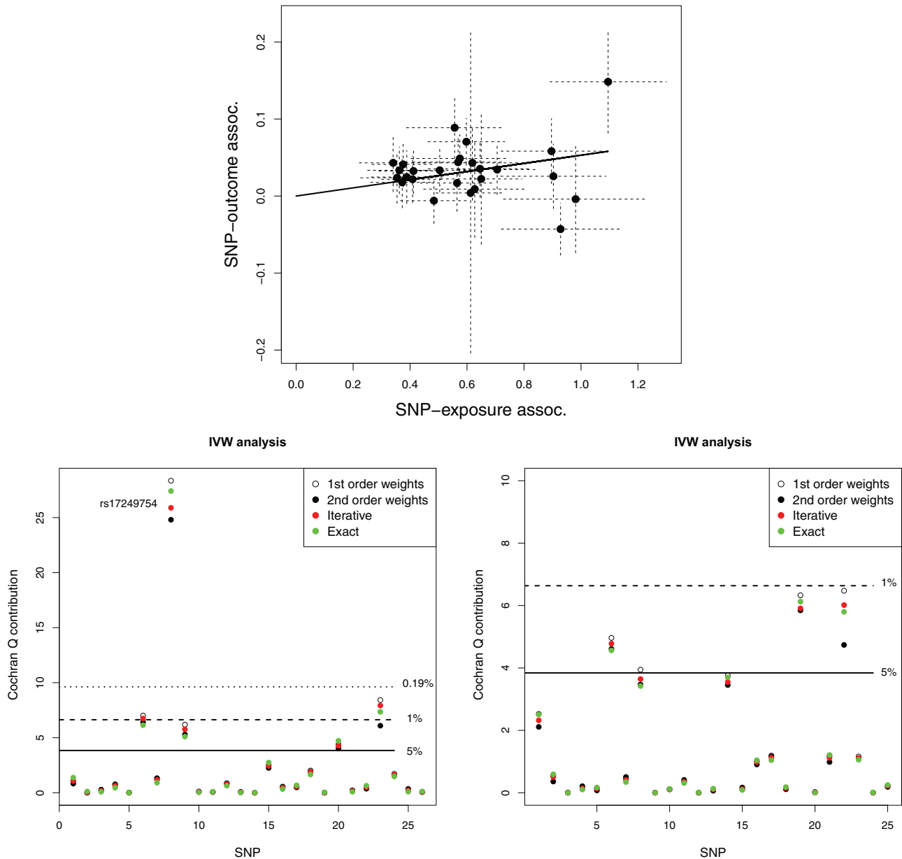
Figure 3. Top: Scatter plot of SNP-outcome associations \hat{\Gamma}_j vs SNP-exposure associations \hat{\beta}_j ; IVW estimate shown as a black slope. Bottom-left: Q contribution plots for the same data. Bottom-right: Q contributions after removal of rs17249754.
