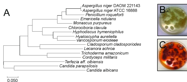
Figure 1. A) Phylogenetic tree of fungal ITS regions showing that Hyphodiscus clusters with fungi from the Leotiomycece family. B) Hyphodiscus grown in the dark. C) Hyphodiscus after being exposed to 12-hour light/dark cycles.
