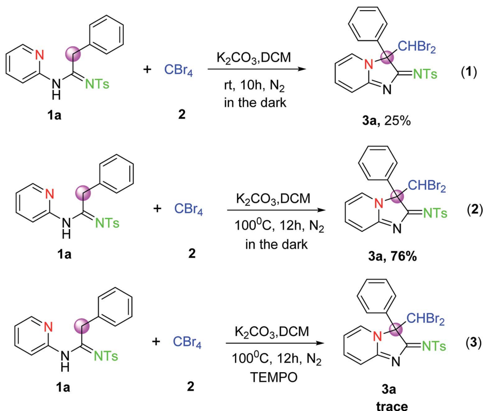
Scheme 2 Control experiments.
